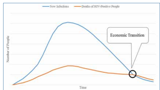
Figure 1: AIDS Transition
